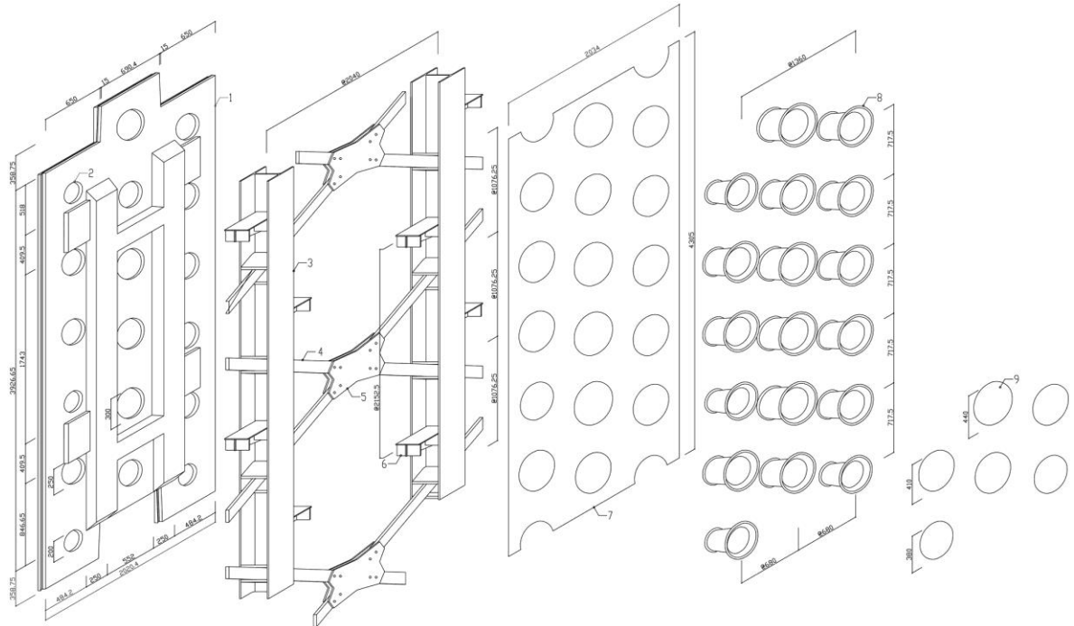
EXTERIOR WALL COMPONENT 1/60
