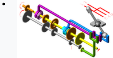
First gear (blue, to back)
