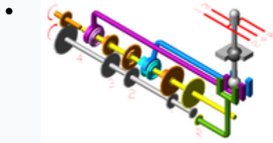
Neutral (blue and purple in the middle, green disengaged)
