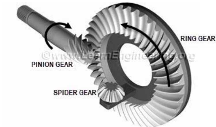
Fig.3 Motion from the pinion gear is transferred to the spider gear
