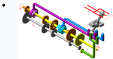
Fourth gear (purple, to front)
