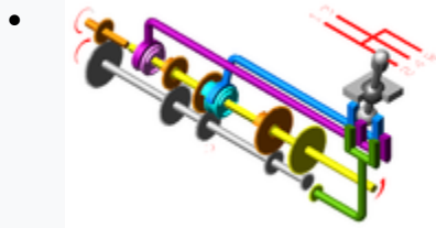
Second gear (blue, to front)
