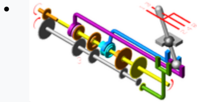
Third gear (purple, to back)
