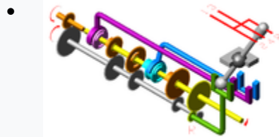
Reverse (green engaged)
